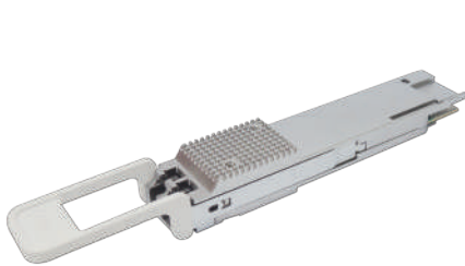
400G QSFP56-DD-ZR/ZR+ DCO
